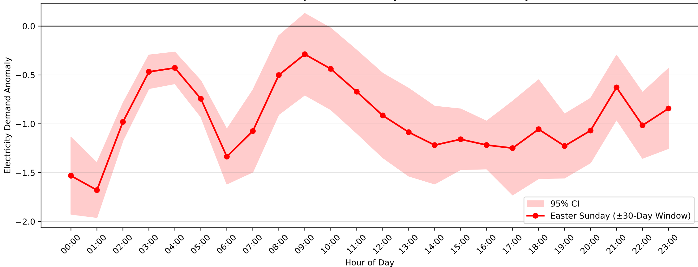
Morisset Demand Anomaly: Easter Sunday (2004-2017, \pm 30 -Day Window)
